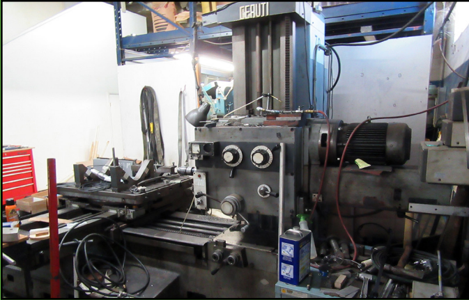
Ceruti Horizontal Boring Mill
