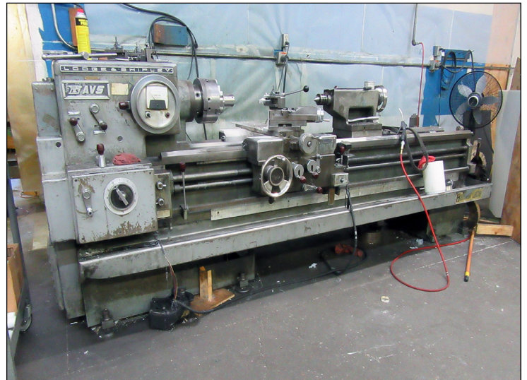
Lodge & Shipley 21" Engine Lathe
