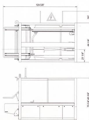
Superformer 1
