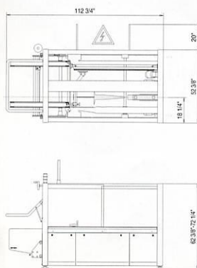
Superformer 1M
