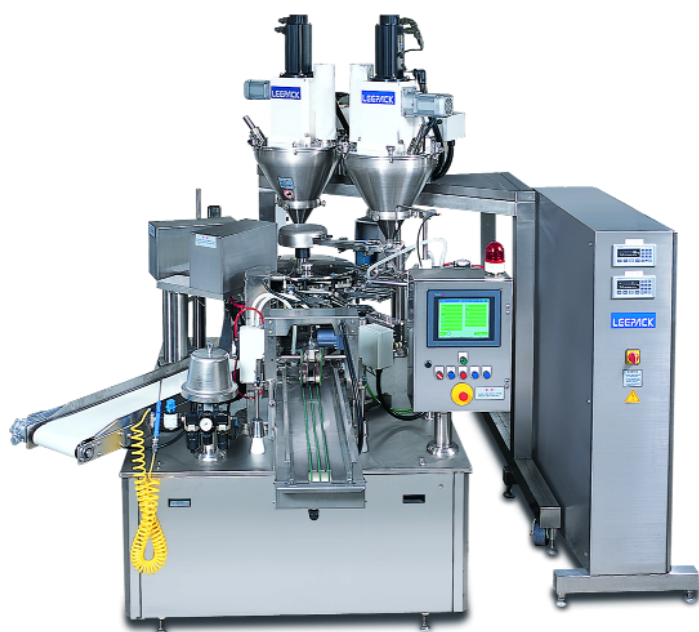
PSG LEE Auger Filling Machine
