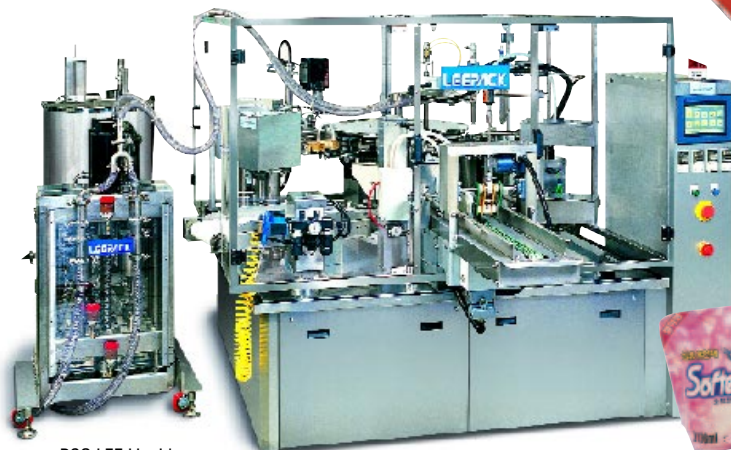
PSG LEE Liquid Fill-Seal Machine
