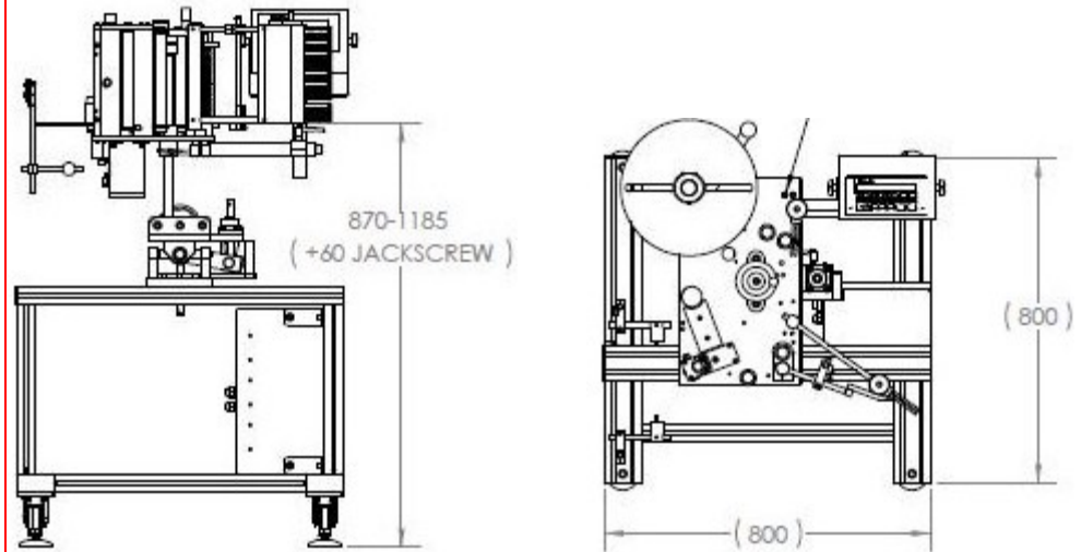
Side Application Footprint (Side view and top view)
