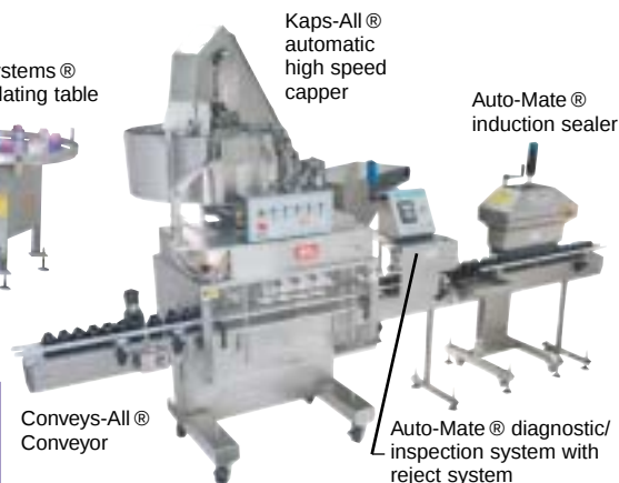
Kaps-All® automatic capper
