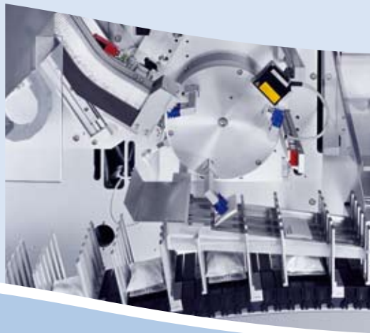
Rotary feeder for inserts
