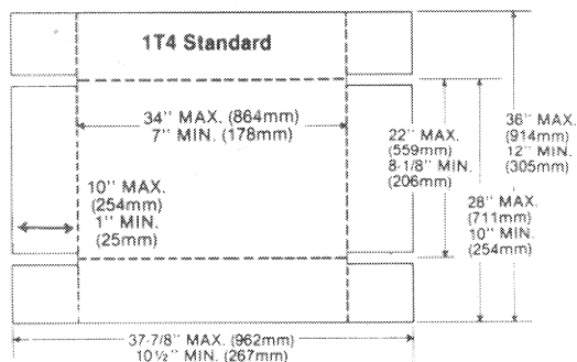
Two-Piece Full Telescope
