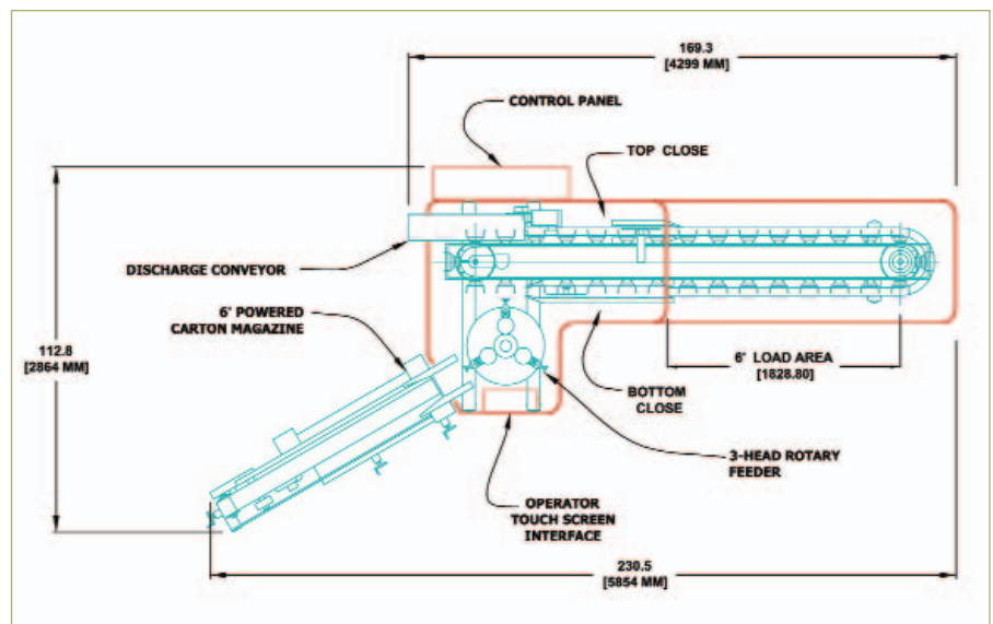
Optional Product Belt Feeder Assembly
