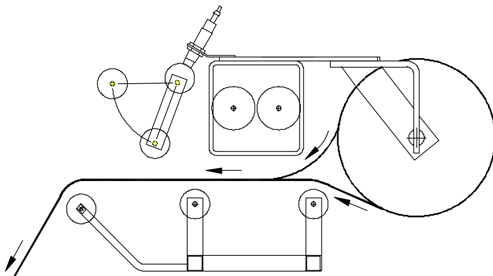
Fig. 1 OPEN CRADLE
