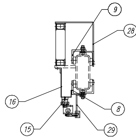
GUARD MOUNTING 1 : 6
