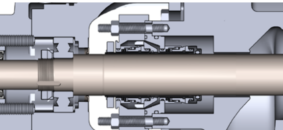
CARTRIDGE - SINGLE OR DUAL
