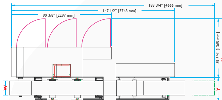
DLI 330 Top View
