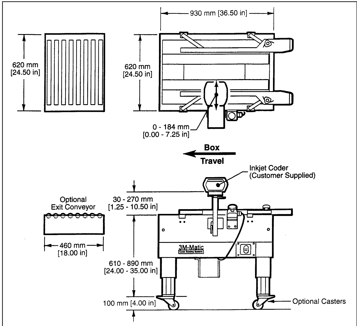
Dimensional Drawing
