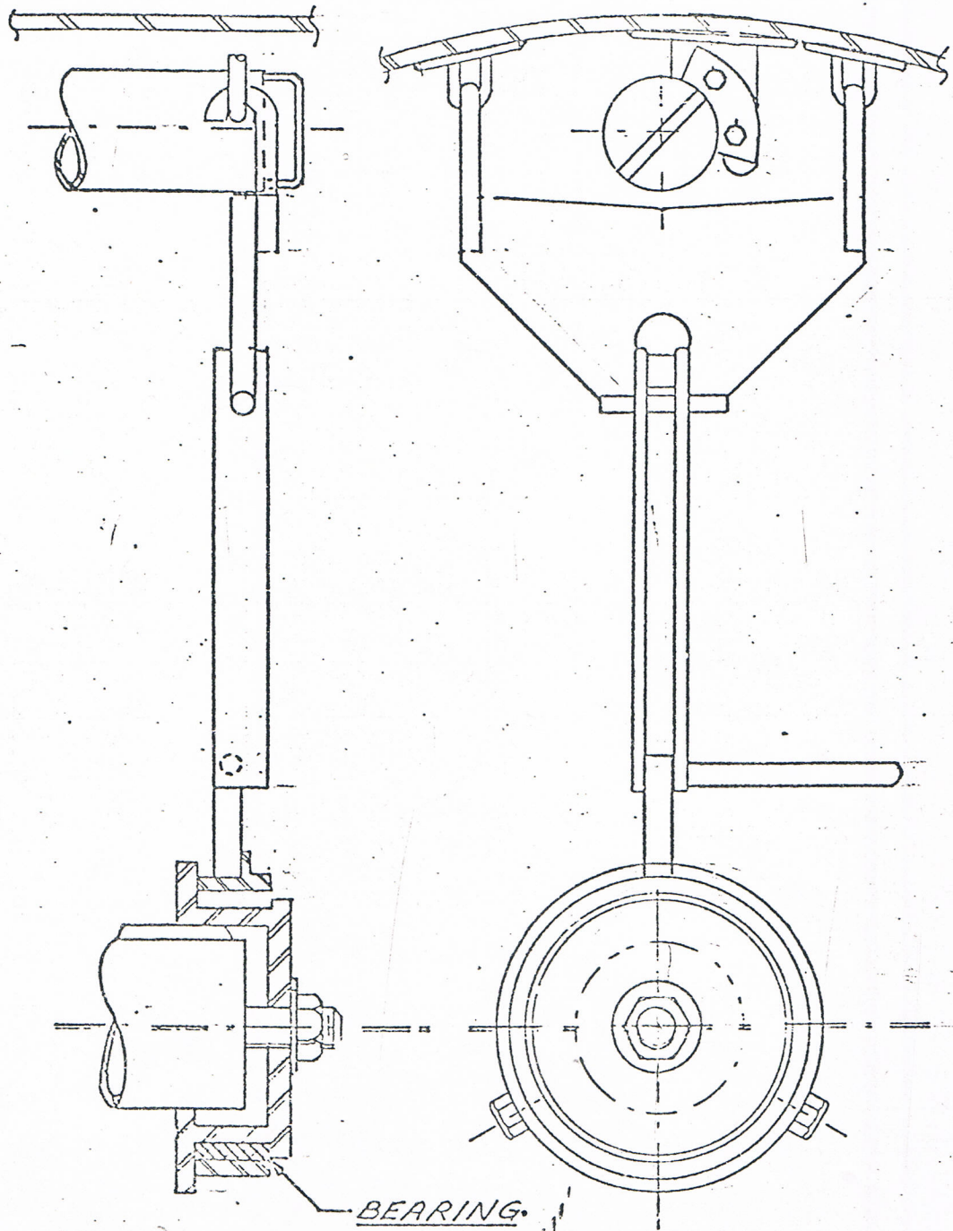
FRONT TOGGLE & BEARING ASSEMBLY
